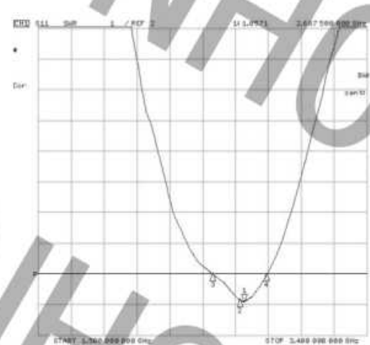
ANT92-2R660G-S1TF
